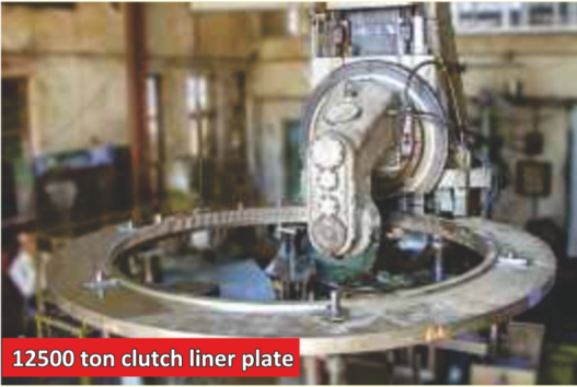
12500 ton press clutch hub and liner and assembly
